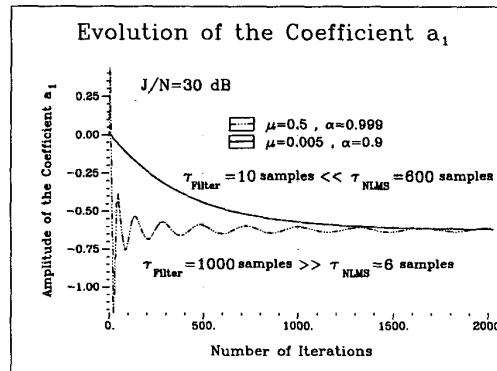
Figure 3-2 Transition Mode of the Adaptation.
