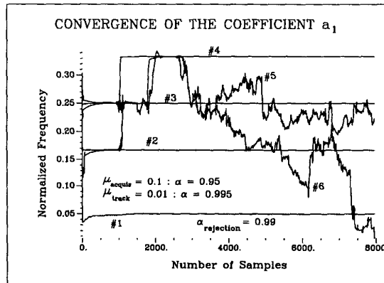
Figure 4-5: Coefficients of the PIRANHA Filter.
