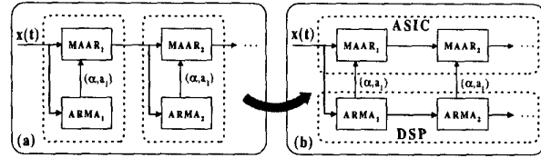
Figure 2-2: From Conventional to PIRANHA Structure.
