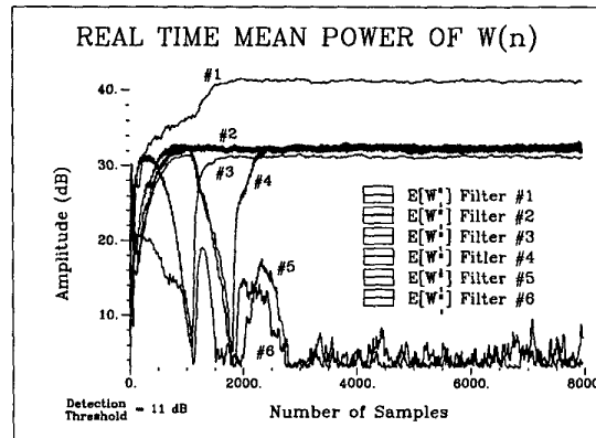
Figure 4-6: Signal w(n) for Cells Activation/Desactivation.
