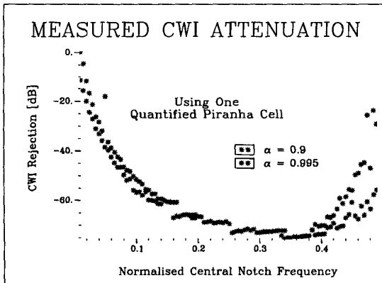
Figure 4-3: Measured CW Interference Attenuation (dB).
