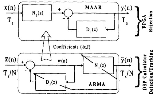
Figure 2-3: Main Structure of the PIRANHA Cell H_1(z) .
