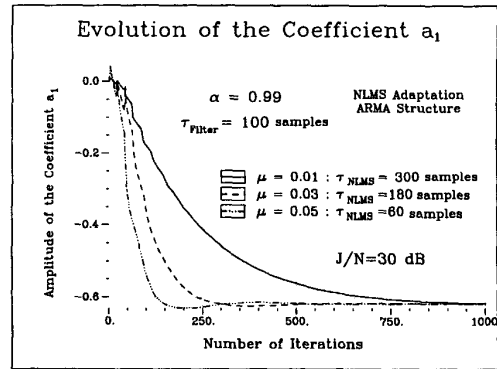
Figure 3-1 Convergence of NLMS Adaptation.
